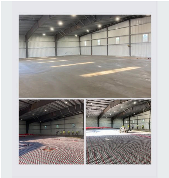
INTERIOR CONCRETE WORK
