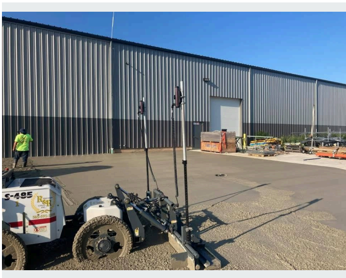
LASER-SCREED PLACEMENT IN ACTION
