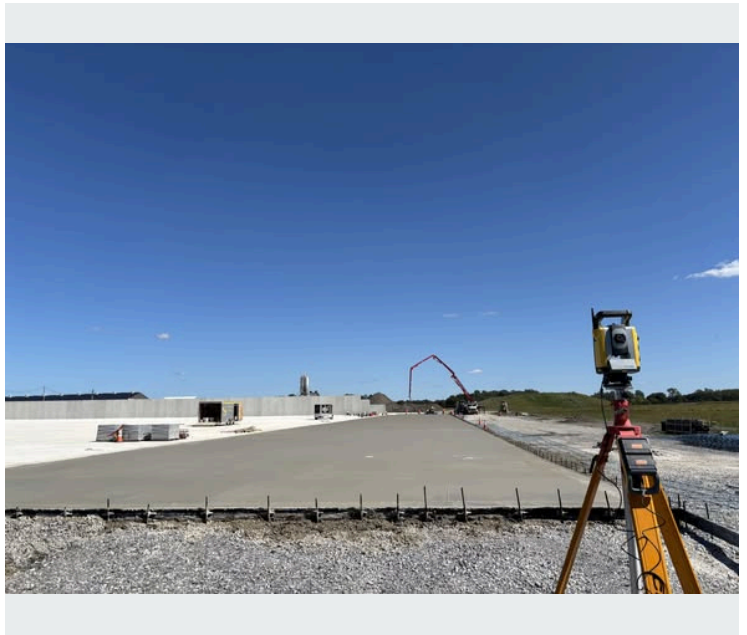
SITE PREPARATION & REINFORCEMENT
