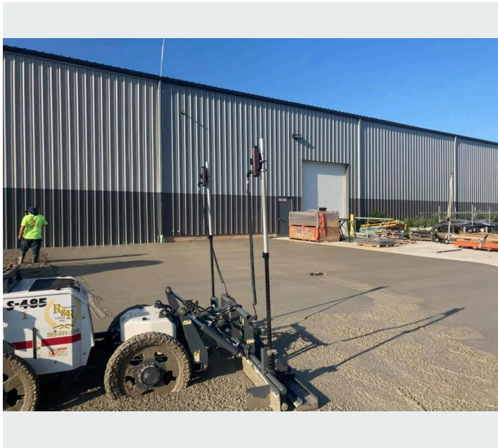
LASER-SCREED CONCRETE PLACEMENT
